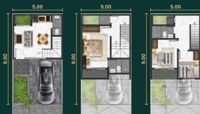
1st FLOOR
