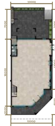
LANTAI 1
