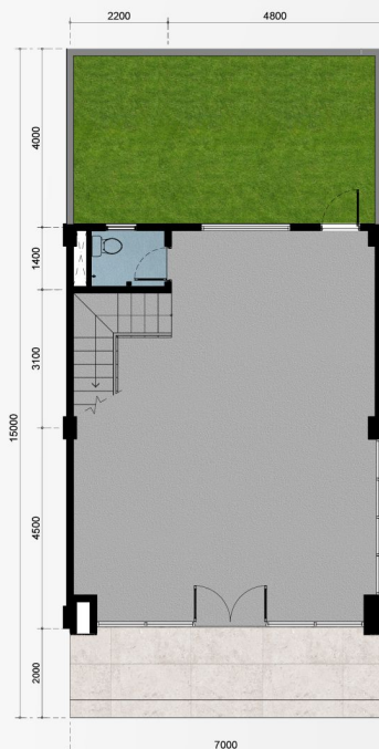
Denah Lantai 1
