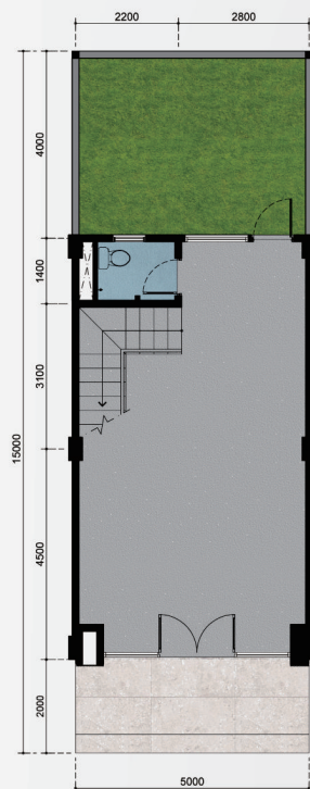
Denah Lantai 1
