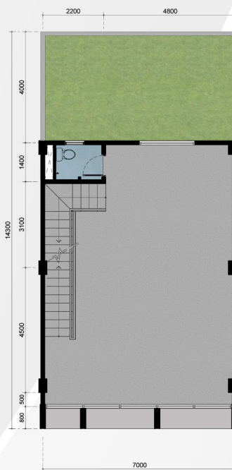
Denah Lantai 2
