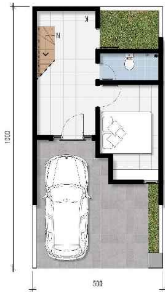
DENAH LT. 1
