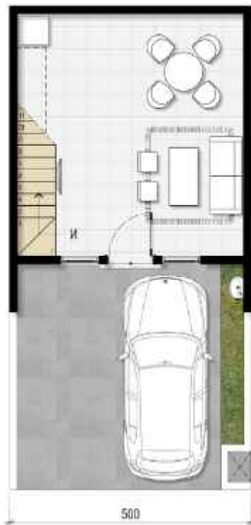
DENAH LT. 1
