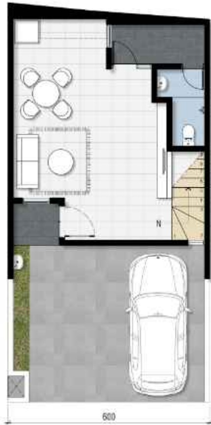
DENAH LT. 1
