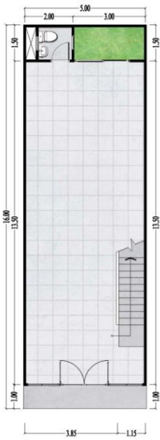
Denah Lantai 1
