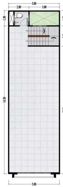
Denah Lantai 3
