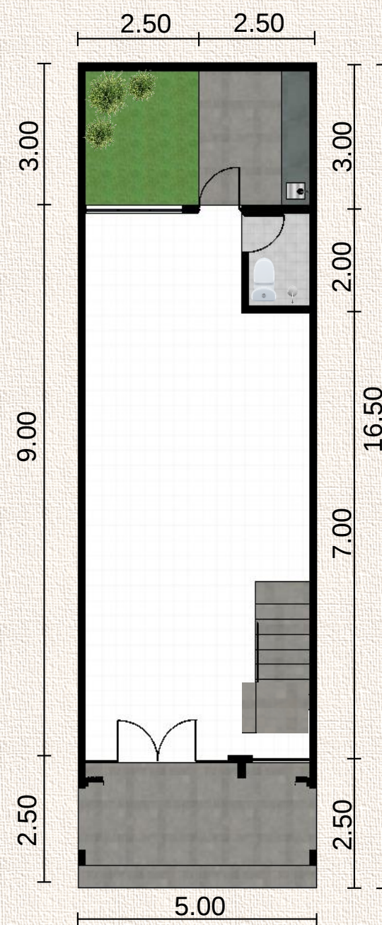
LANTAI 1
