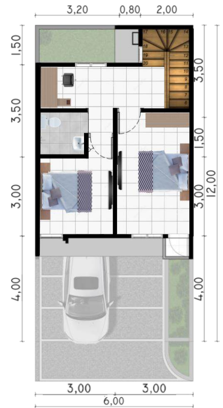
Denah Lantai 2
