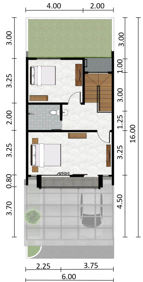
Denah Lantai 2
