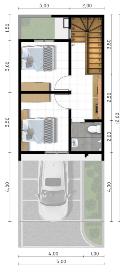
Denah Lantai 2
