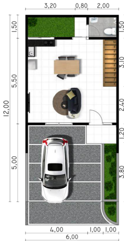
Denah Lantai 1
