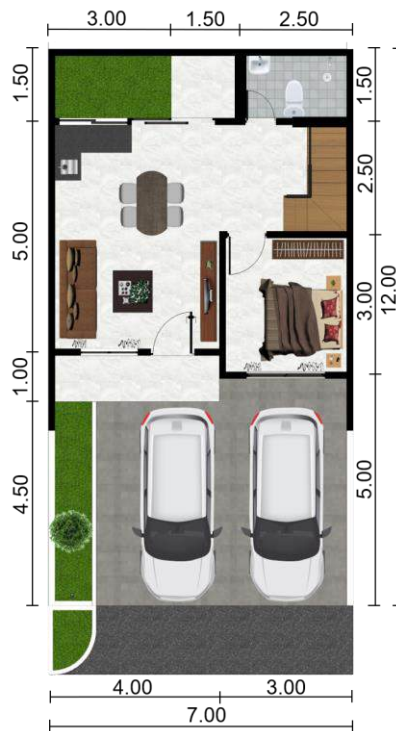
Denah Lantai 1
