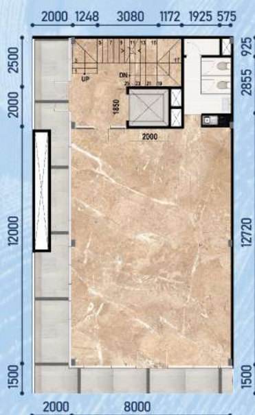
Denah lantai dasar
