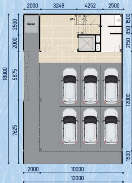
Denah lantai semi-basement
