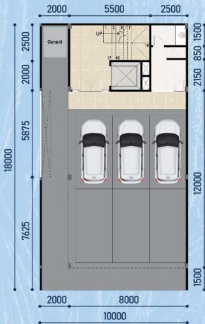
Denah lantai semi-basement
