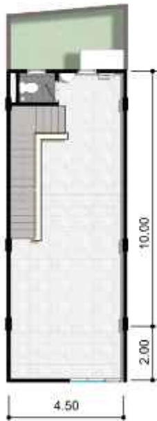
DENAH LT.2
