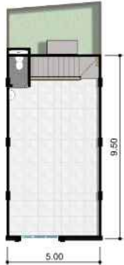
DENAH LT.2
