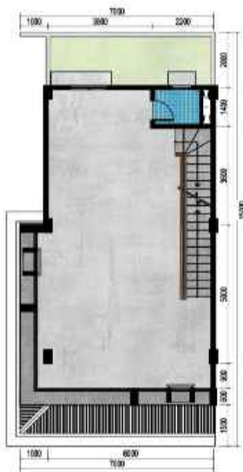
Denah Lantai 2
