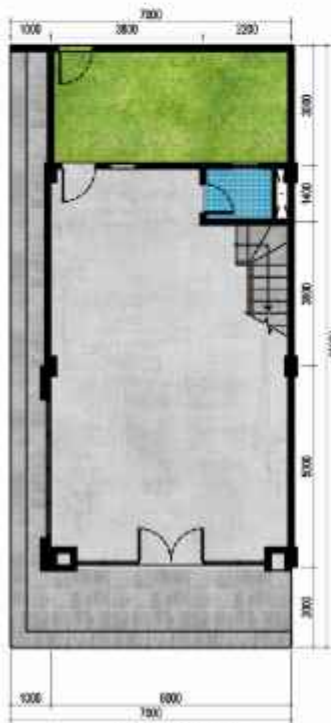
Denah Lantai 1
