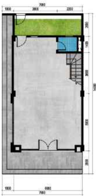
Denah Lantai 1
