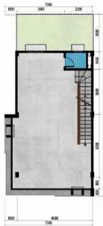
Denah Lantai 3
