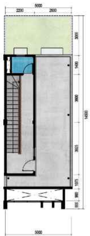
Denah Dak Atap
