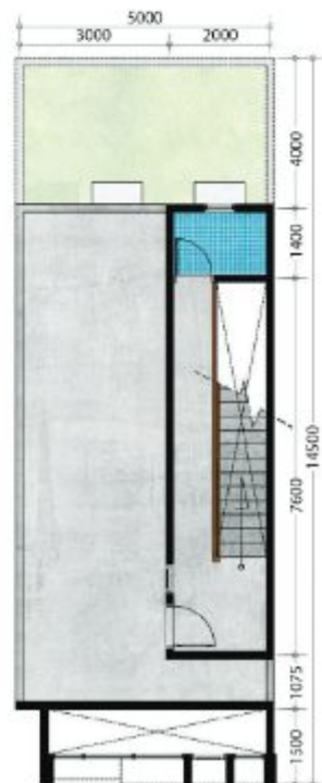
ROOF FLOOR
