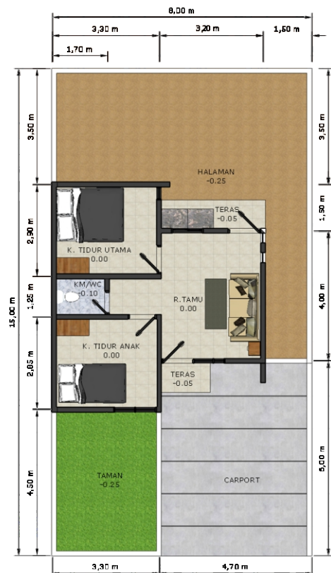
DENAH TIPE 36/120 *Tanpa Pagar Keliling
