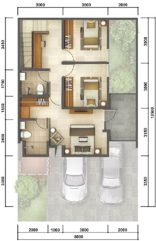
DENAH LANTAI 2
