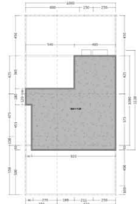
Lantai Atap
