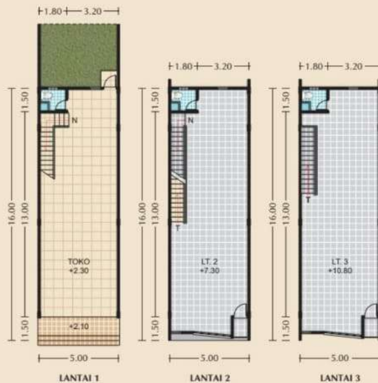
RUKO 3 LANTAI - T.244 (A18,19,22,23,24)
