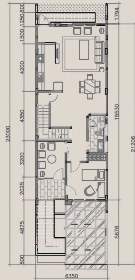
G FLOOR
