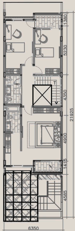
2ND FLOOR
