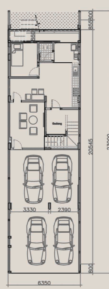
LG FLOOR
