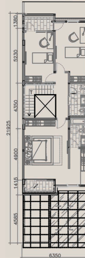
2 ND FLOOR
