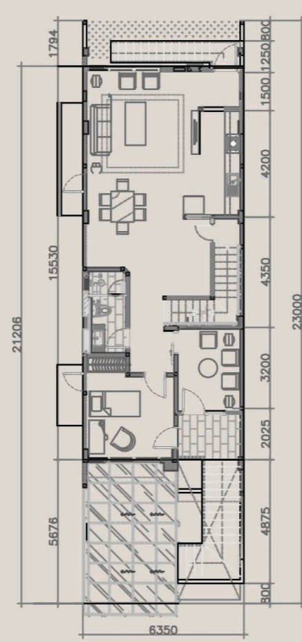
G FLOOR
