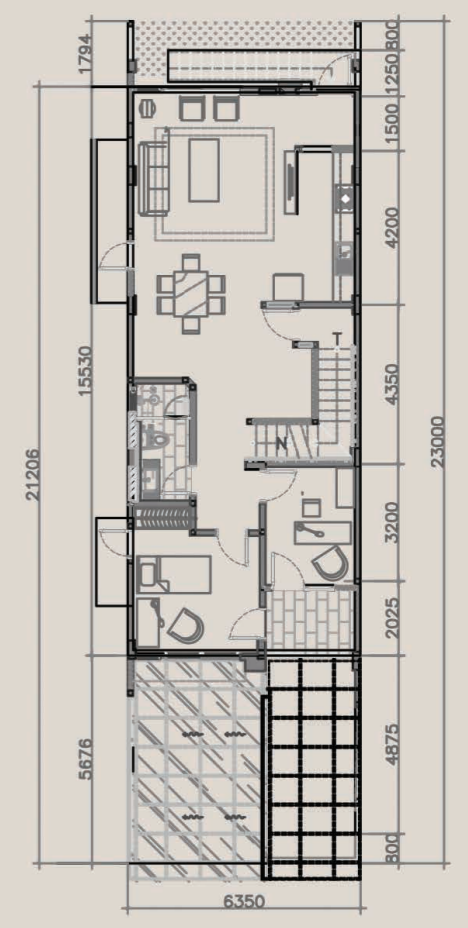
G FLOOR
