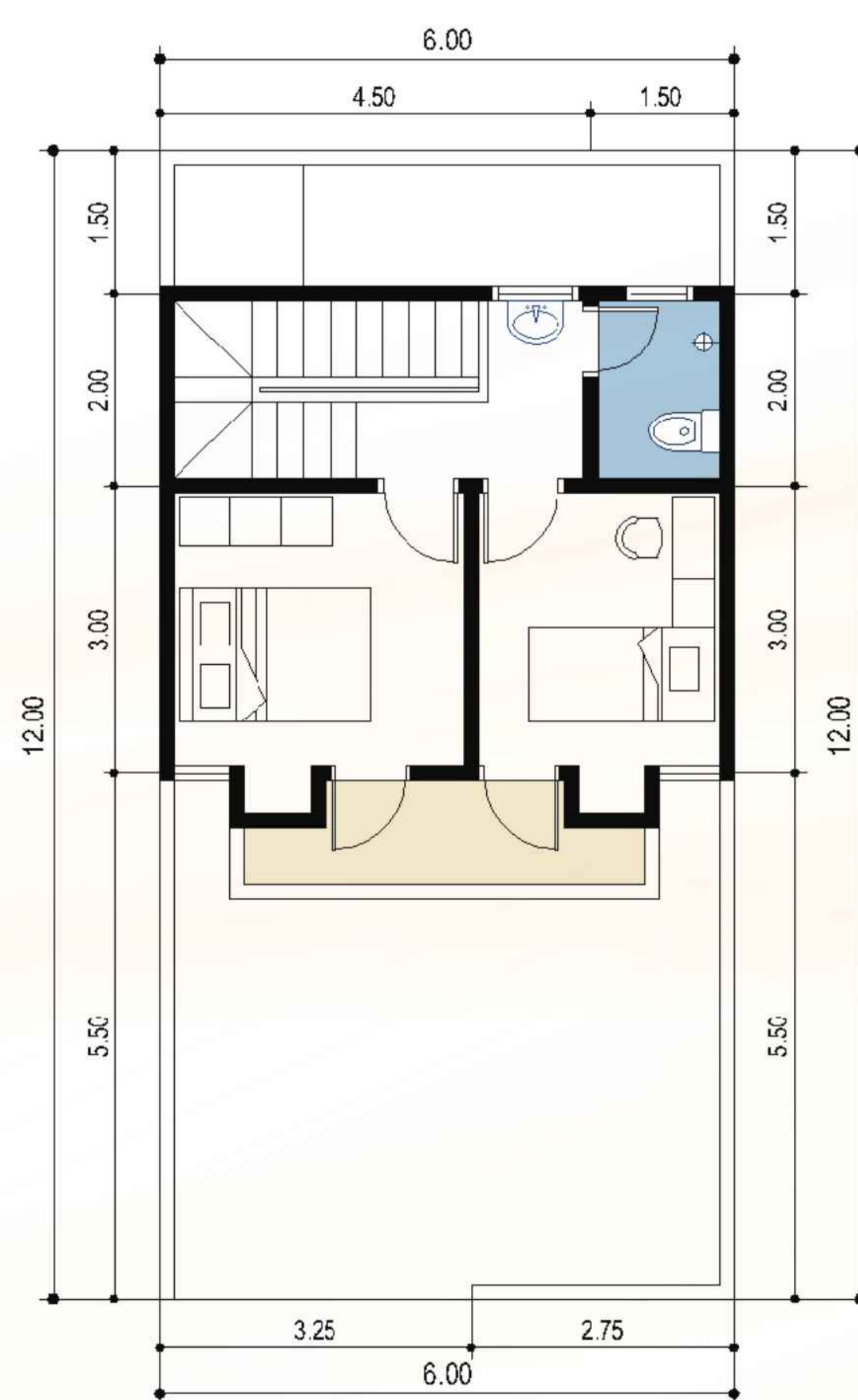
DENAH LANTAI 2
