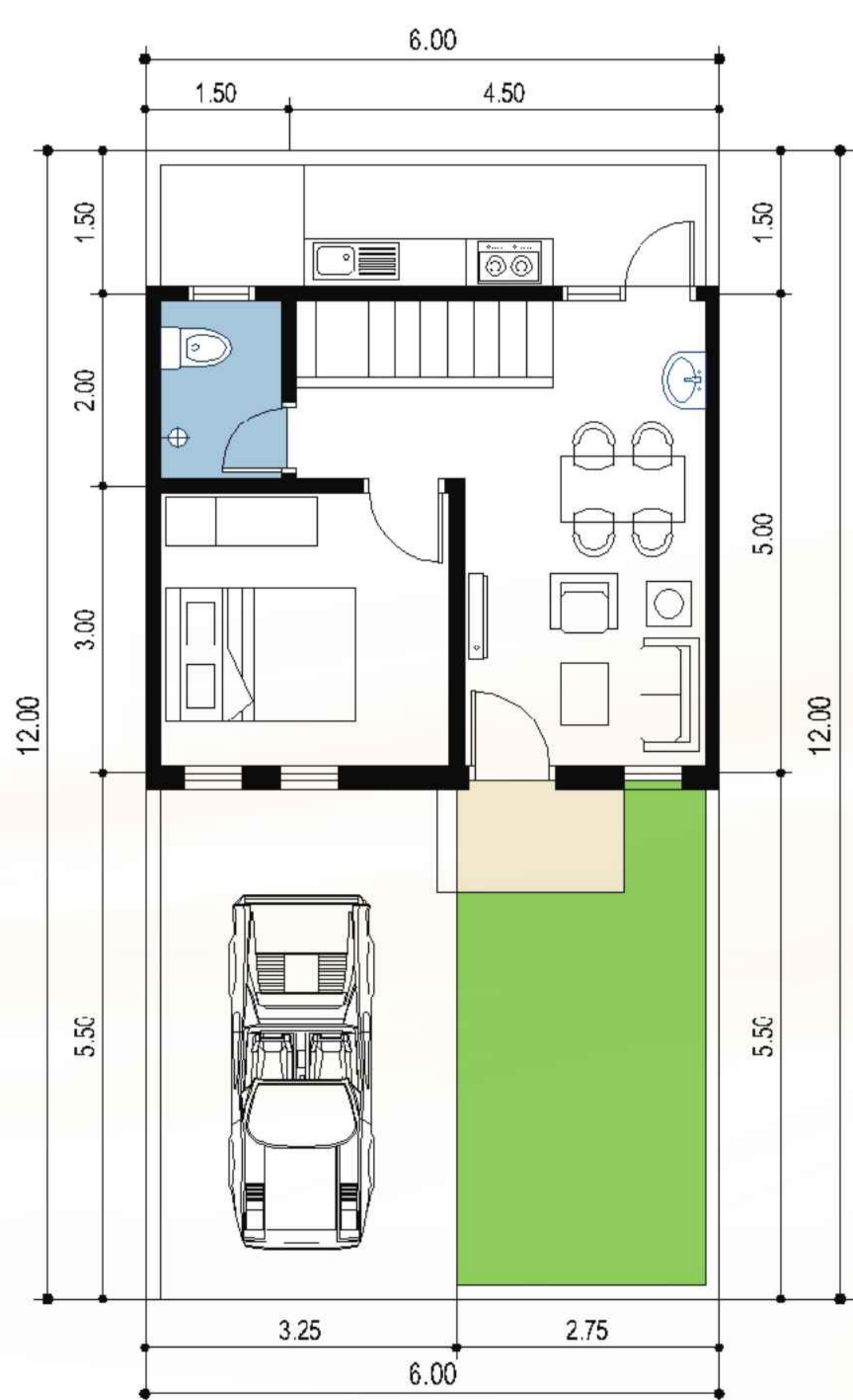
DENAH LANTAI 1
