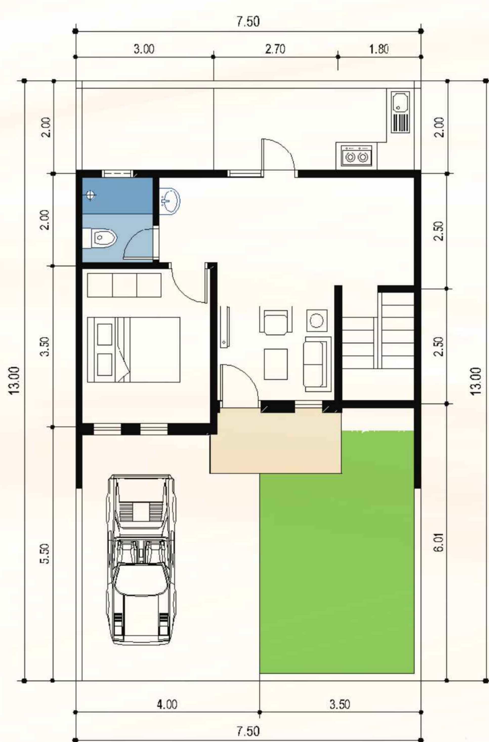
DENAH LANTAI 1
