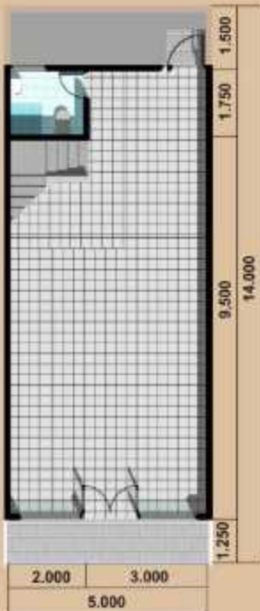
DENAH LANTAI DASAR
