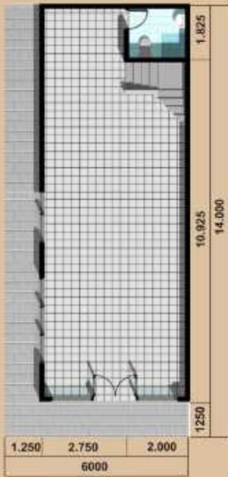
DENAH LANTAI DASAR
