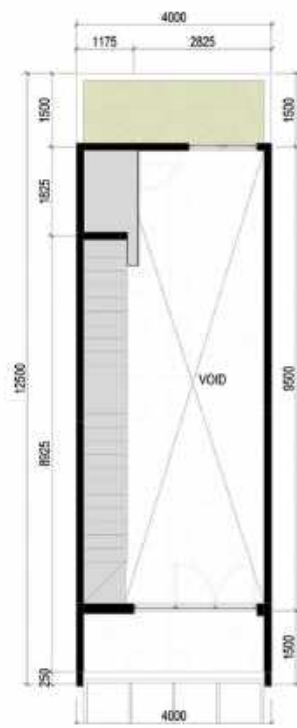
DENAH LANTAI MEZZANINE
