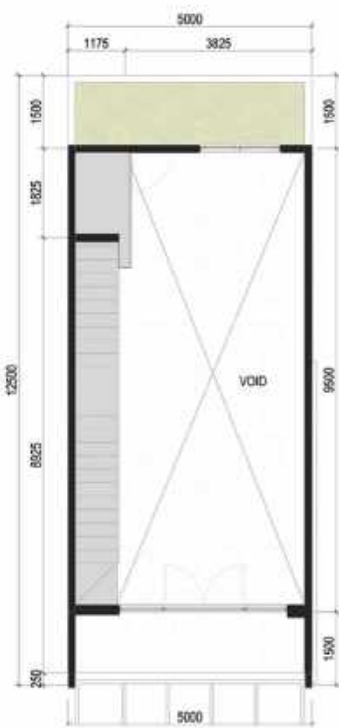
DENAH LANTAI MEZZANINE
