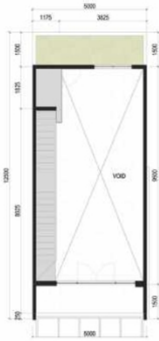
DENAH LANTAI MEZZANINE
