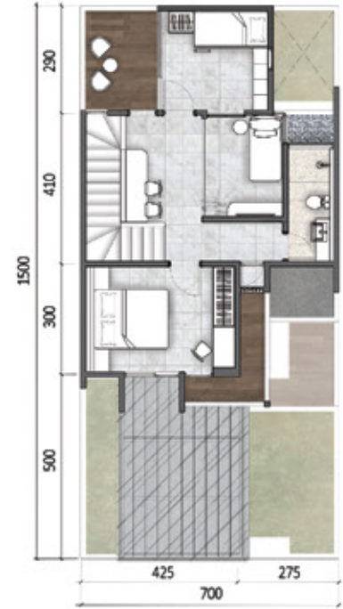
Denah Lantai 2
