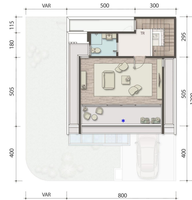
LANTAI ATTIC
