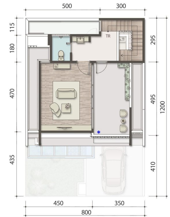
LANTAI ATTIC
