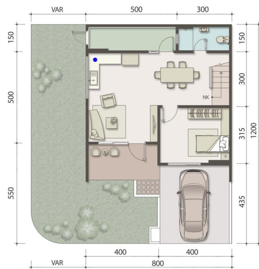
LANTAI 1
