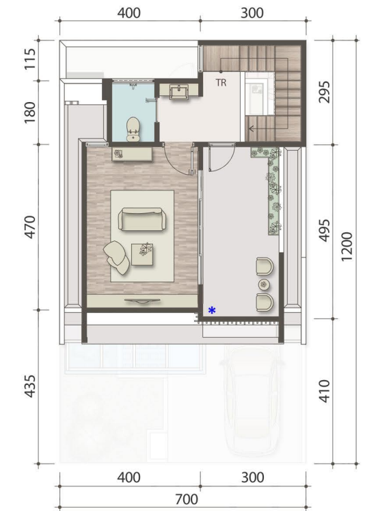
LANTAI ATTIC
