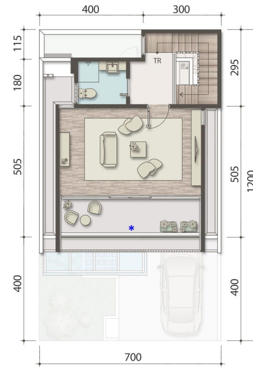
LANTAI ATTIC
