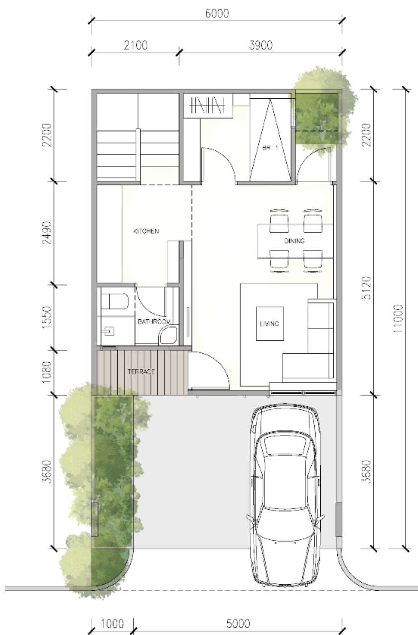
Ground Floor
