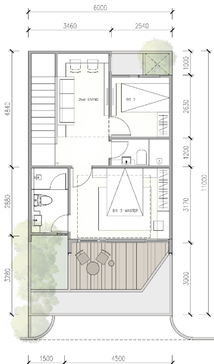
Second Floor
