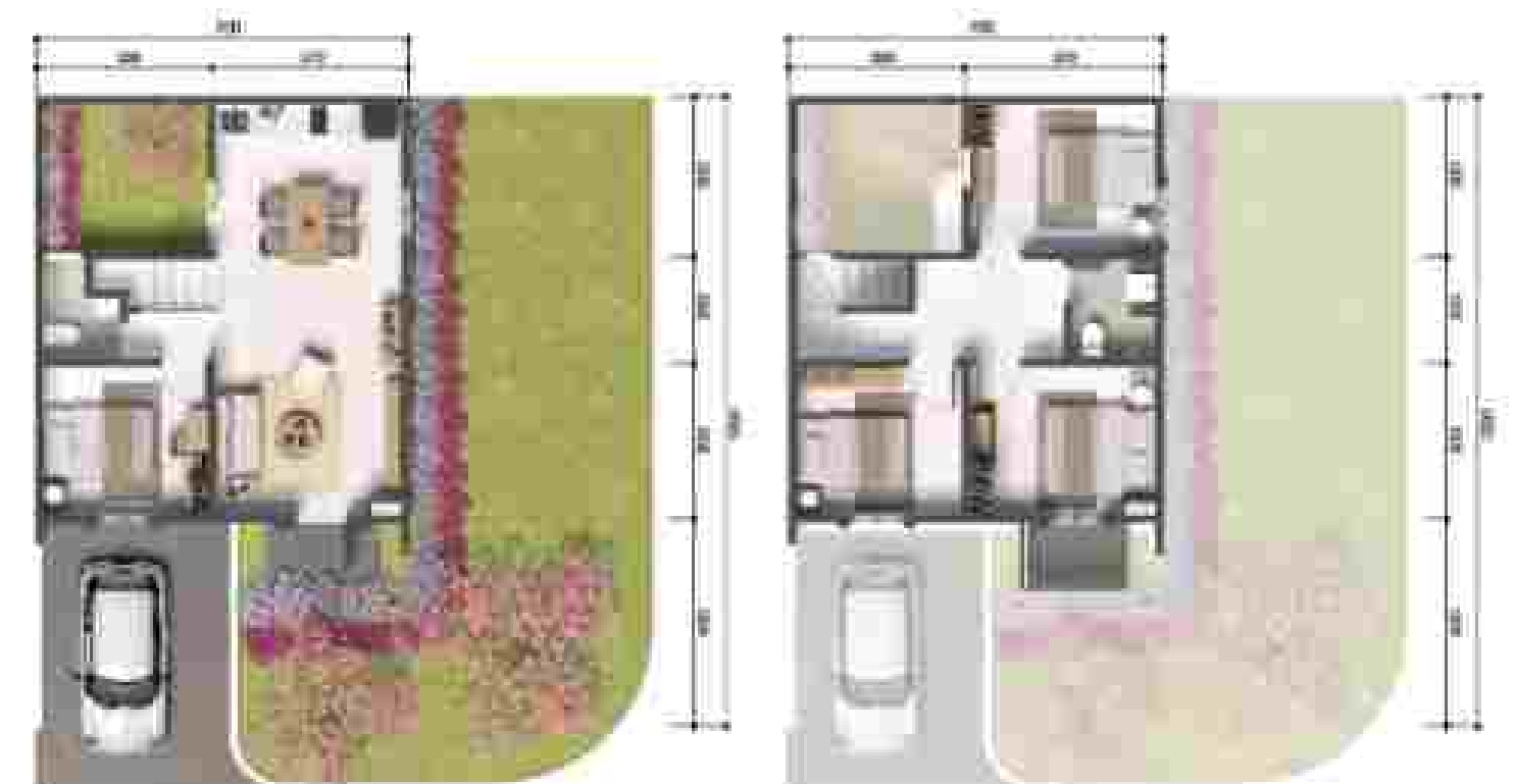
Lantai 1
