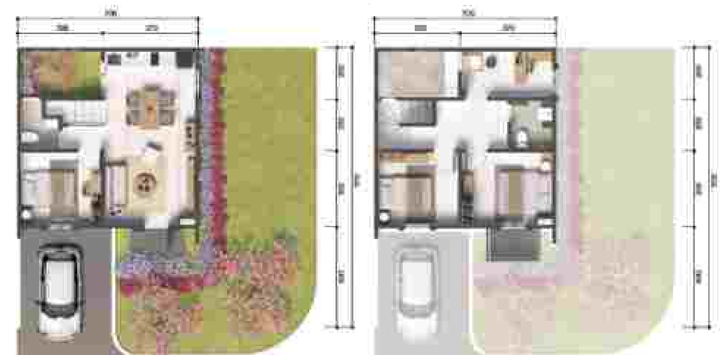
Lantai 1
