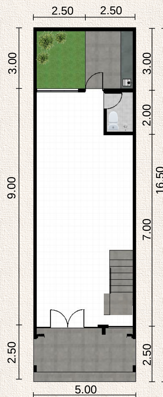
LANTAI 1
