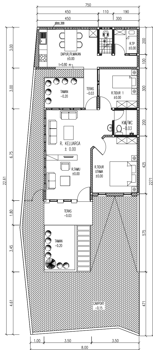
DENAH Luas = 93 m 2
