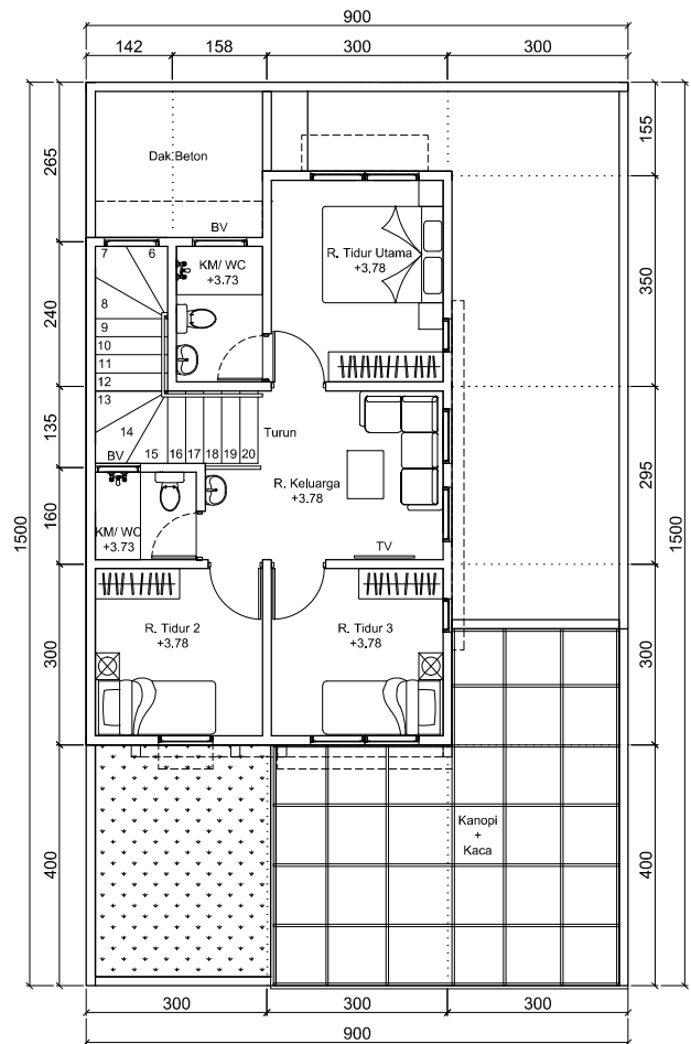
DENAH LANTAI 2 55 m 2
