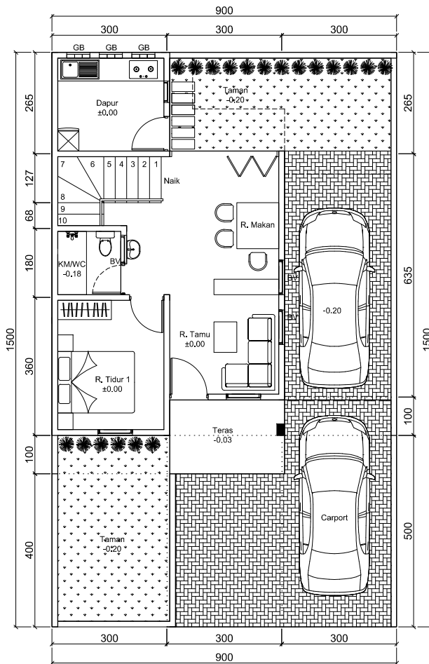
DENAH LANTAI 1 53 m 2
