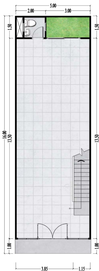
Denah Lantai 1
