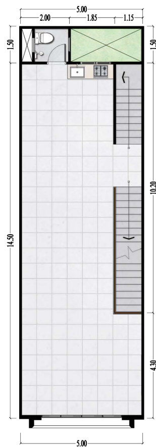
Denah Lantai 2
